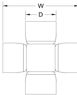
TYPE TWO OUTSIDE SNAP RINGS
